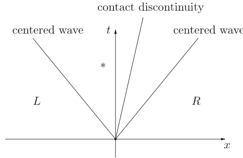
Figure 2. Structure of the Riemann problem.
